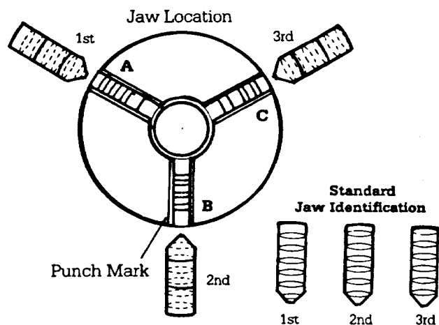
FIGURE 1—Three-Jaw Chuck, standard jaw locations.
